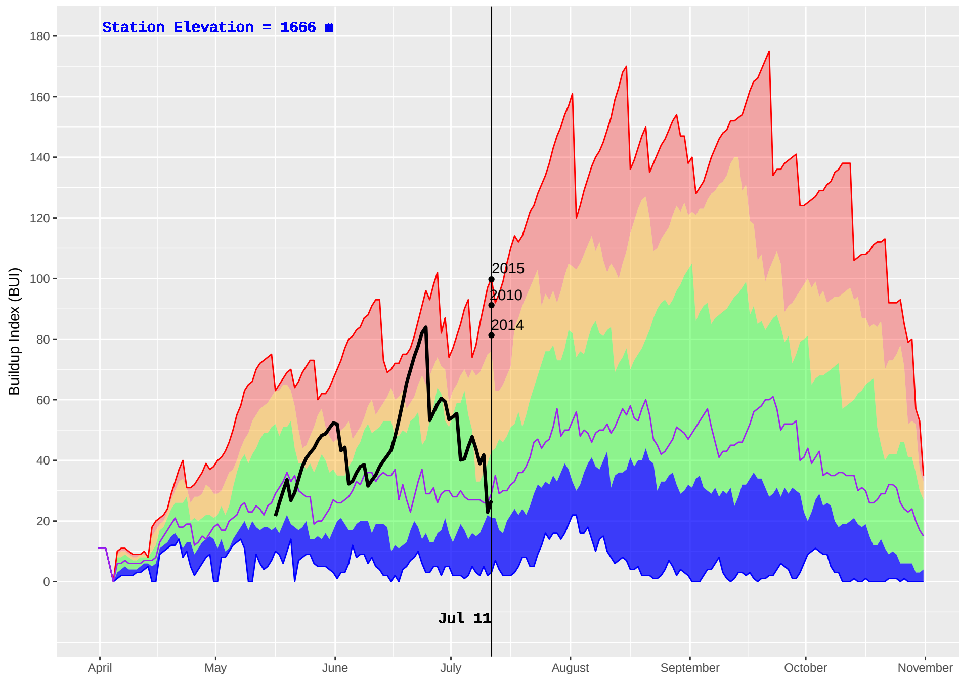
BALDFACE (221) : Historical (1992–2016) and Current (2018) Noon Buildup Index (BUI)
