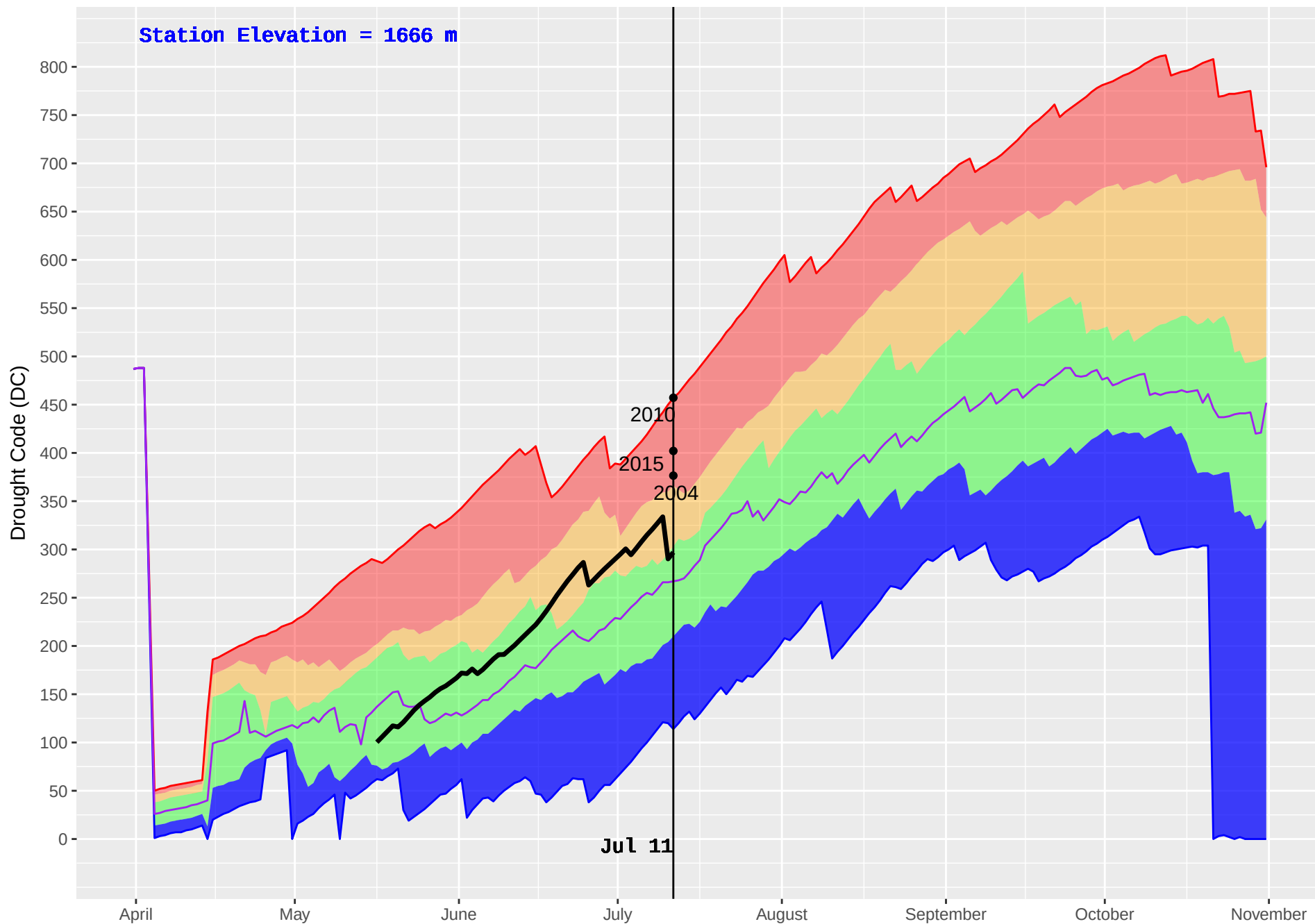
BALDFACE (221) : Historical (1992–2016) and Current (2018) Noon Drought Code (DC)
