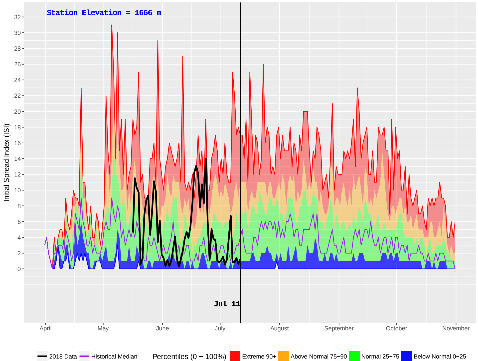
BALDFACE (221) : Historical (1992–2016) and Current (2018) Noon Initial Spread Index (ISI)
